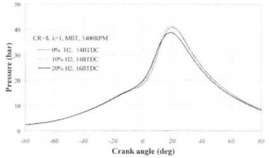
Fig. 4 Cylinder pressure versus crank angle at 1400 RPM, MBT, and a compression ratio of 8 with various H 2 proportions
