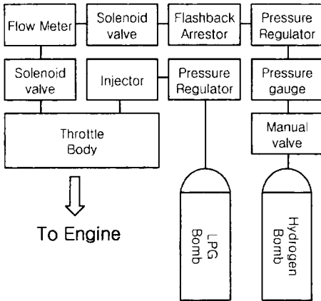
Fig. 3 The fuel supply system
