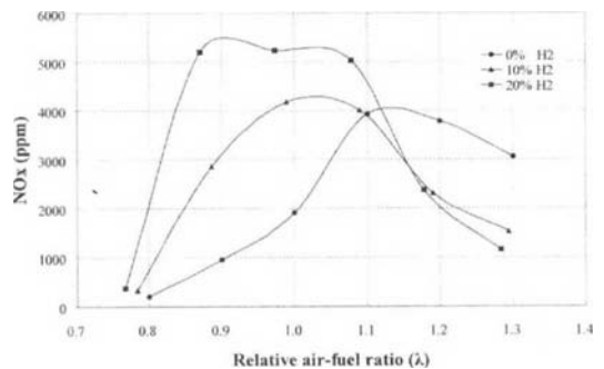
Fig. 8 NOx emission versus relative air-fuel ratio for hydrogen rates
