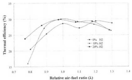
Fig. 9 Thermal efficiency versus relative air-fuel ratio for the addition hydrogen
