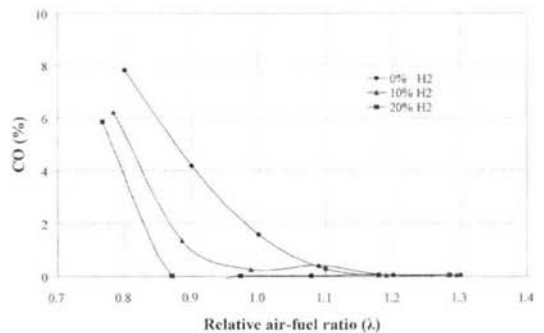
Fig. 6 CO emission versus relative air-fuel ratio for different hydrogen rates
